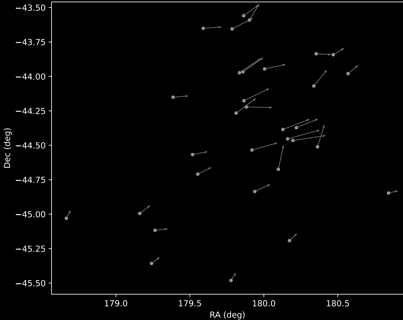
GALAH DR4 Cluster 14 Proper Motion Vectors (n=32)
