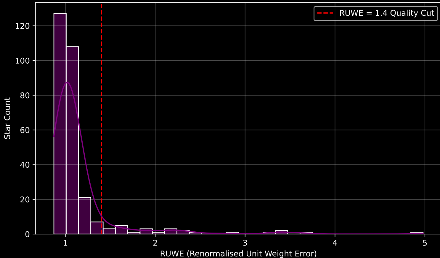
GALAH DR4 Field [559] RUWE Distribution (n= 288)
