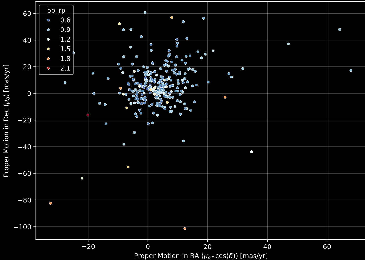
GALAH DR4 Field: [559] Proper Motion Diagram (n= 300)
