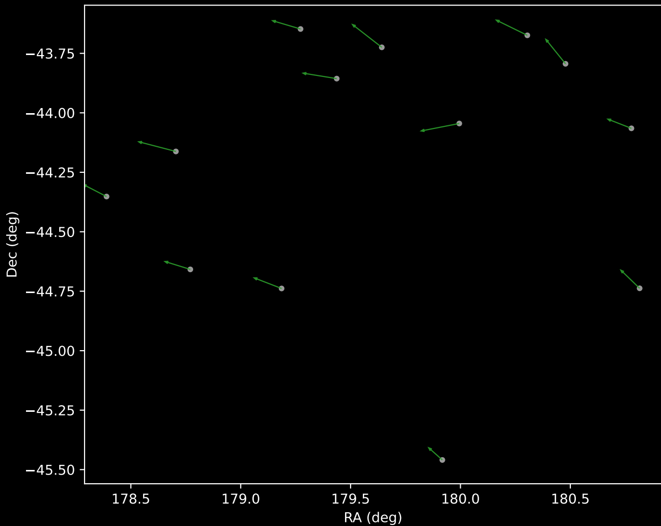
GALAH DR4 Cluster 4 Proper Motion Vectors (n=13)
