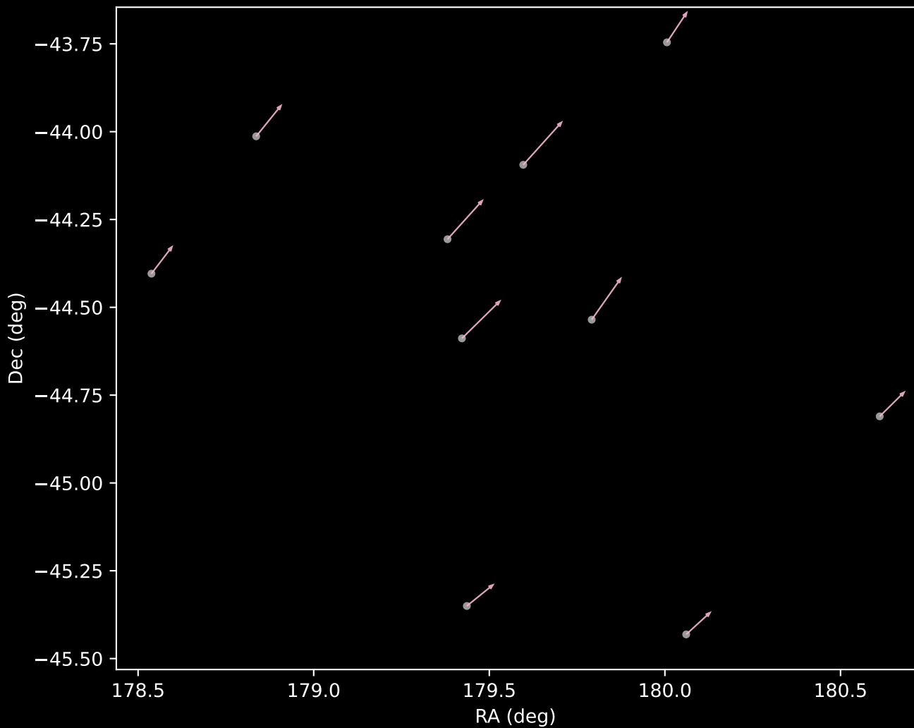
GALAH DR4 Cluster 13 Proper Motion Vectors (n=10)
